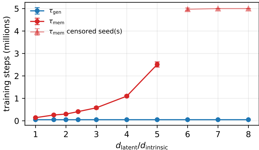
5-seed mean timescales with 95% CI
